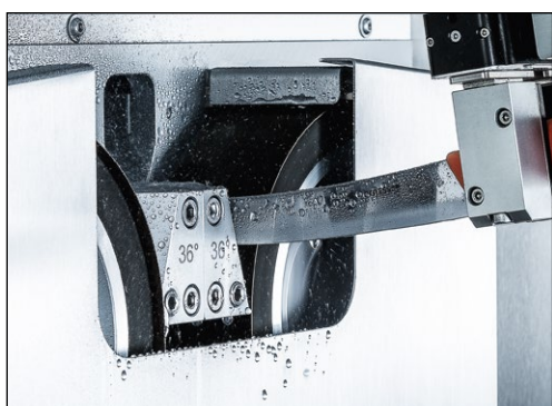
Figure 7-6 Grinding hand knives
