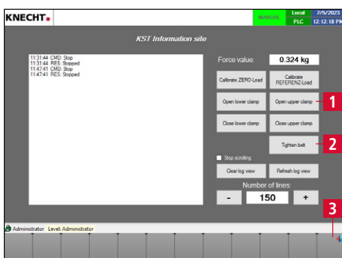
Figure 7-71 Settings sharpness testing device
