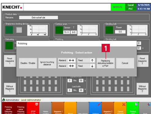
Figure 7-38 Polishing – Replacing the polishing rings
