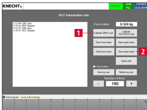
Figure 7-65 Calibrating "ZERO-Load"
