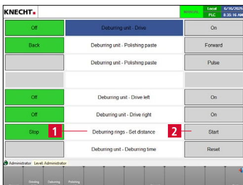
Figure 7-36 Adjusting the deburring rings
