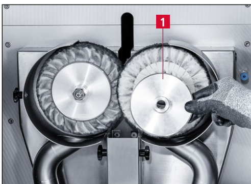
Figure 7-42 Removing the flange washer
