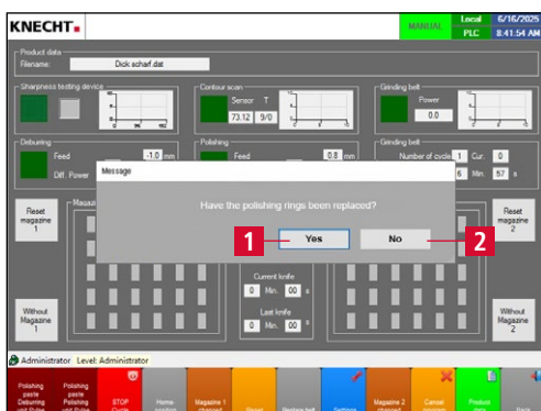
Figure 7-51 Message "Have the polishing rings been replaced?"
