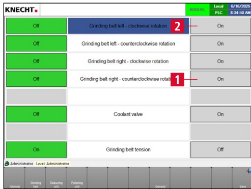
Figure 7-19 Manual functions "Grinding belt"
